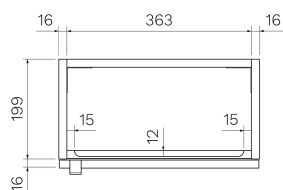
TOP VIEW (CABINET ONLY)
