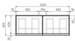
INTERNAL VIEW
