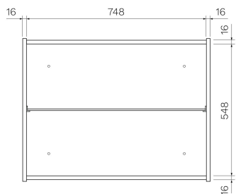
INTERNAL VIEW
