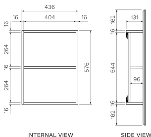
INTERNAL VIEW
