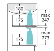
SIDE VIEW: RECESS & DRAWER STORAGE
