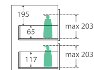
SIDE VIEW: DRAWER STORAGE
