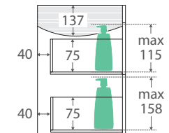
SIDE VIEW: RECESS & DRAWER STORAGE
