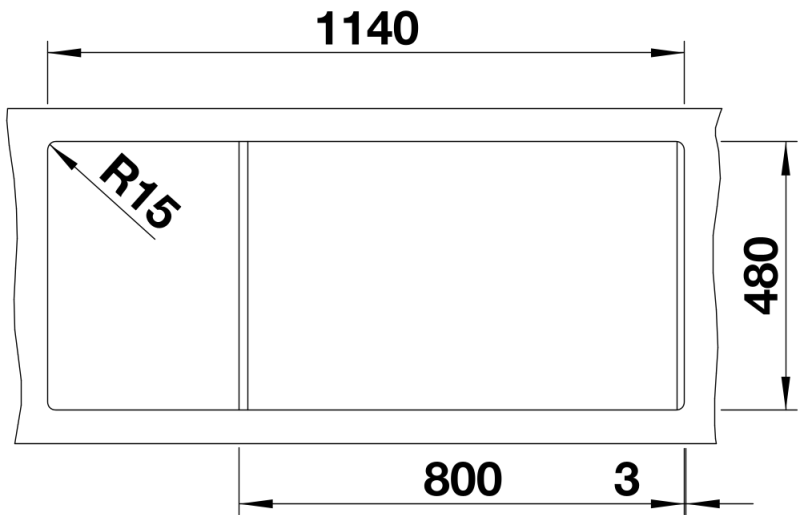
Cut-out
