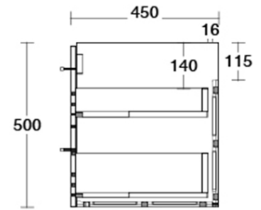
Side Section
