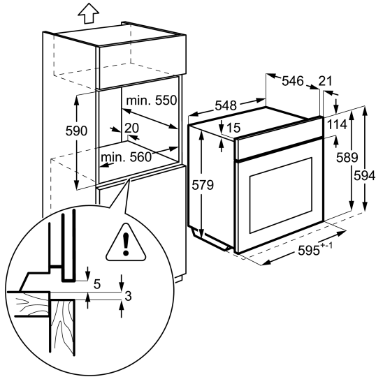
Model: BEK435020B CABINET INSTALLATION
