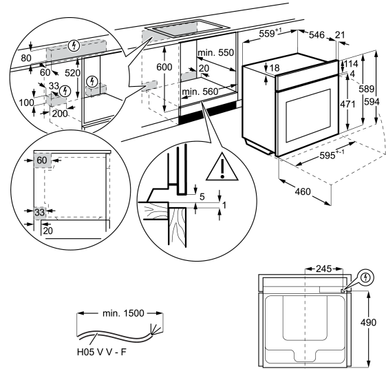
Model: BEK435020B UNDERBENCH INSTALLATION
