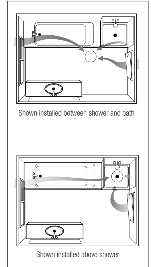
Fig. 4: Ideal placement of Eco Ventflo. Sufficient air inlets into room are required.
