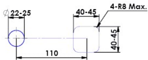
Mounting Hole
