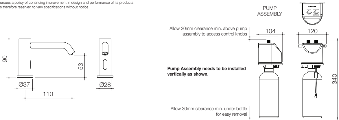
Figure 1: Overall Dimensions
