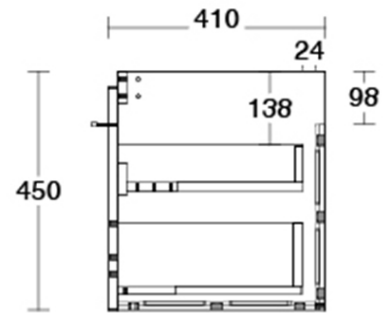
Side Section
