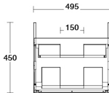
Front Section
